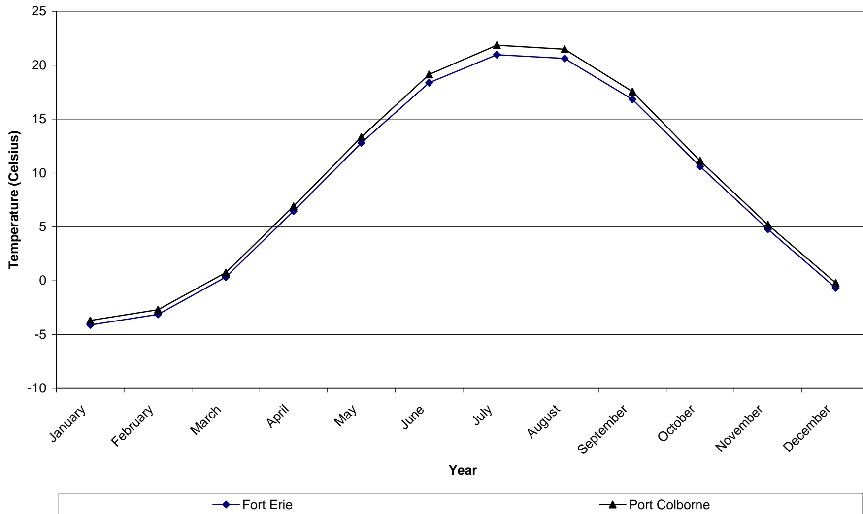
FIGURE 2.3 MEAN (1991-2005) MONTHLY TEMPERATURE FEC WATERSHED PLAN AREA
