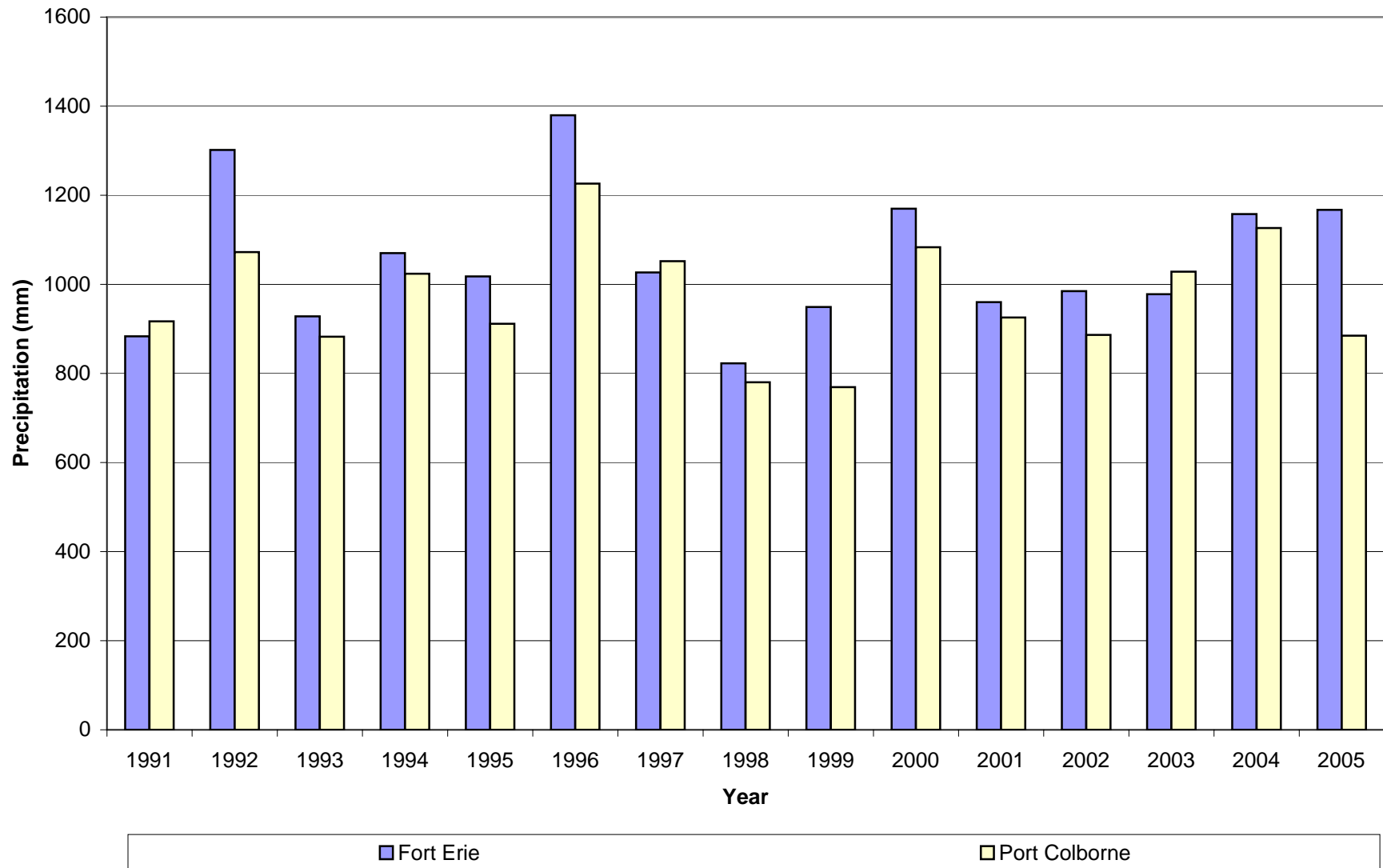
Figure 2.7 ANNUAL PRECIPITATION FEC WATERSHED PLANNING AREA
