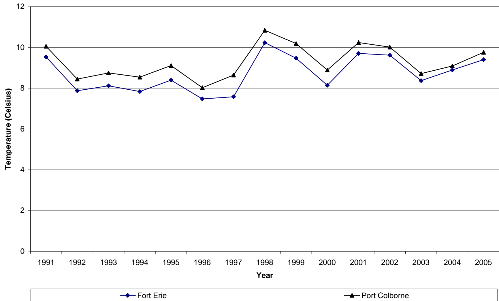
FIGURE 2.9 MEAN (1991-2005) ANNUAL TEMPERATURE FEC WATERSHED PLAN AREA
