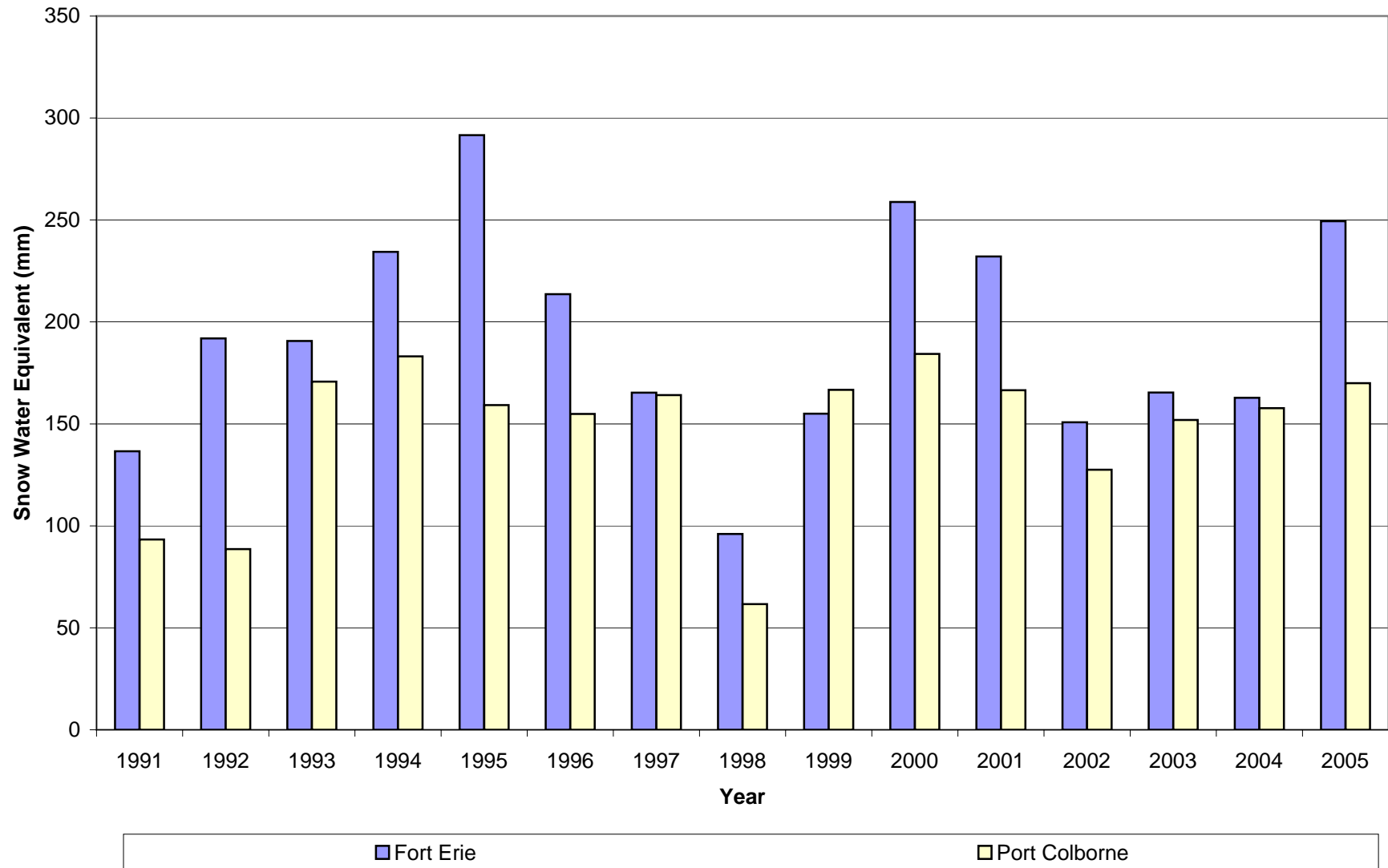
FIGURE 2.8 ANNUAL SNOW WATER EQUIVALENT FEC WATERSHED PLANNING AREA
