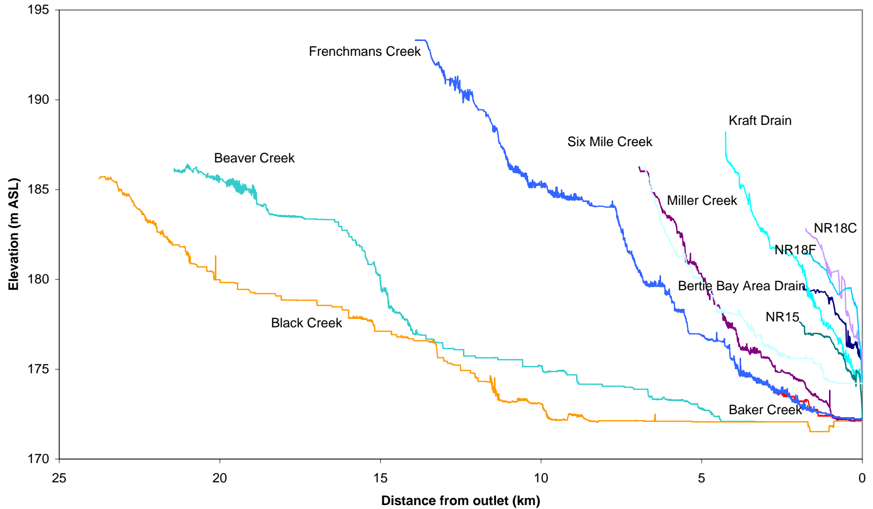
Figure 2.12 Channel Profiles for Fort Erie Watershed Planning Area
