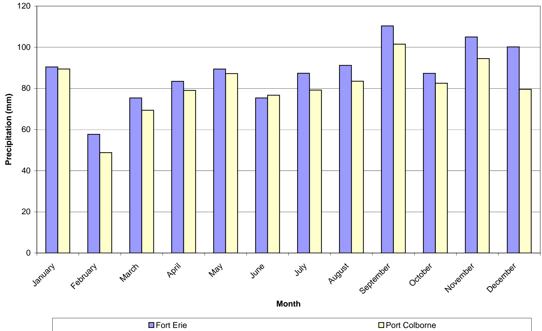
FIGURE 2.2 MEAN (1991-2005) MONTHLY PRECIPITATION FEC WATERSHED PLANNING AREA
