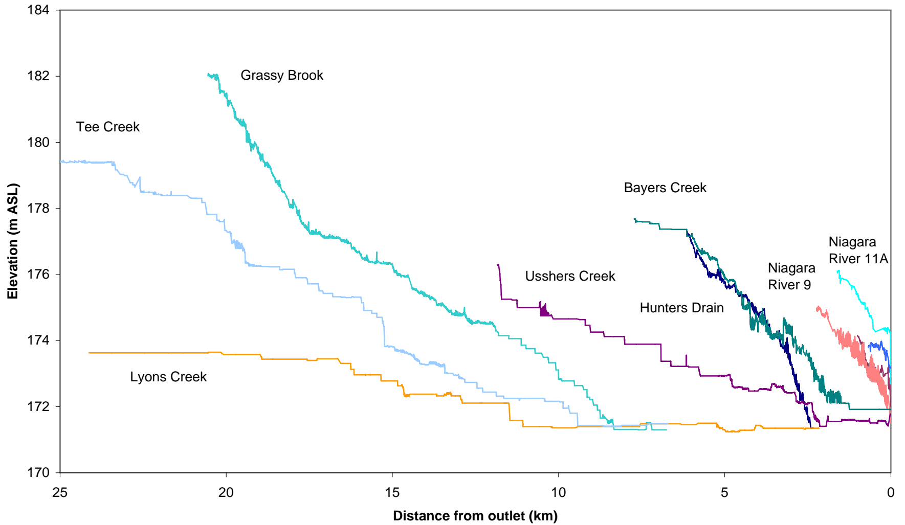
Figure 2.12a Channel Profiles for South Niagara Falls Watershed Planning Area
