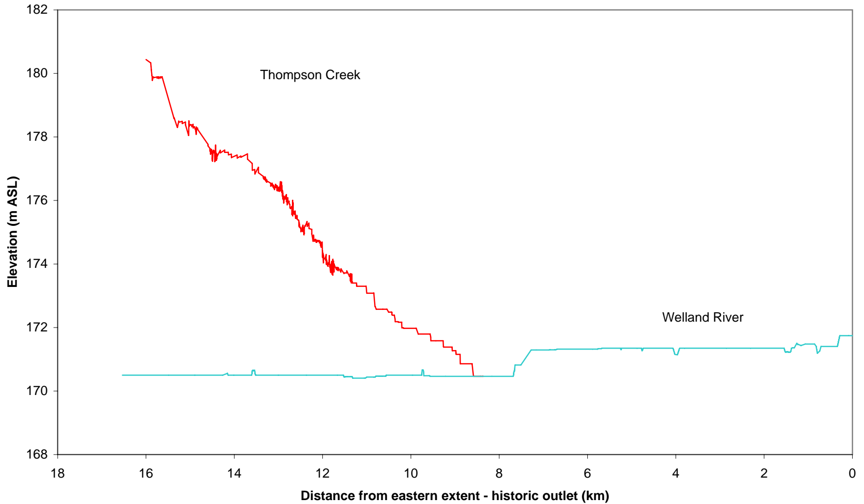
Figure 2.12b Channel Profiles for Lower Welland River Watershed Planning Area
